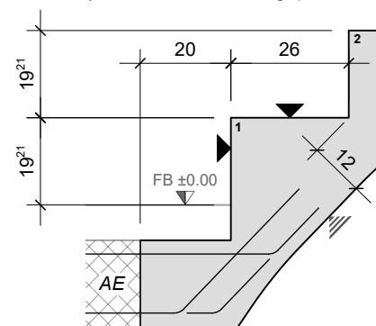
DETAIL A ANTRITT
