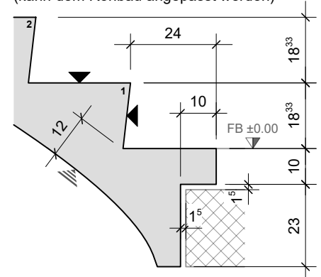
DETAIL A ANTRITT
