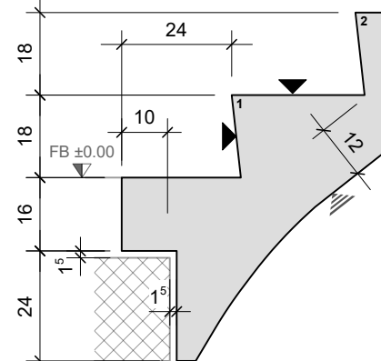
DETAIL A ANTRITT
