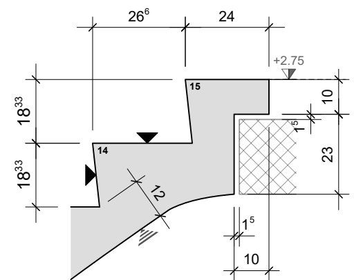
DETAIL C AUSTRITT
