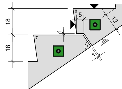
DETAIL A ANTRITT
