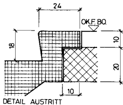
DETAIL AUSTRITT
