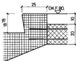
DETAIL AUSTRITT
