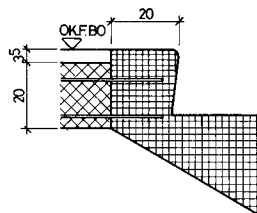
DETAIL AUSTRITT
