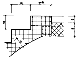
DETAIL AUSTRITT
