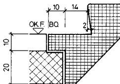
DETAIL ANTRITT
