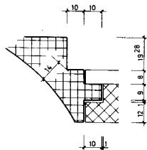
DETAIL AUSTRITT
