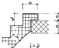
DETAIL AUSTRITT
