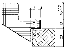
DETAIL ANTRITT
