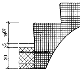
DETAIL ANTRITT
