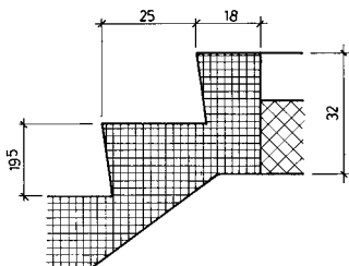
DETAIL AUSTRITT
