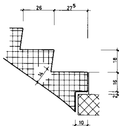
DETAIL ANTRITT
