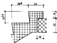
DETAIL AUSTRITT
