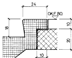
DETAIL AUSTRITT
