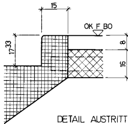
DETAIL AUSTRITT
