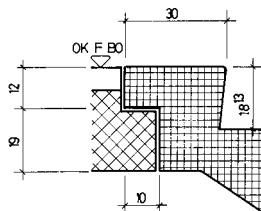
DETAIL AUSTRITT
