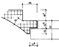
DETAIL ANTRITT
