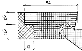
DETAIL AUSTRITT
