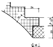
DETAIL ANTRITT
