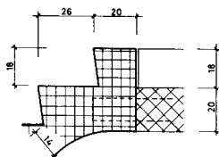
DETAIL AUSTRITT
