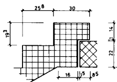
DETAIL AUSTRITT
