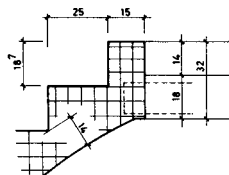
DETAIL AUSTRITT
