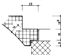
DETAIL ANTRITT
