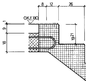
DETAIL AUSTRITT
