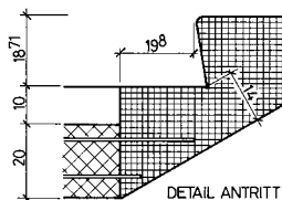
DETAIL ANTRITT
