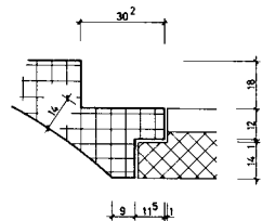
DETAIL ANTRITT
