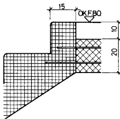
DETAIL AUSTRITT
