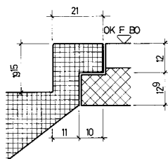
DETAIL AUSTRITT
