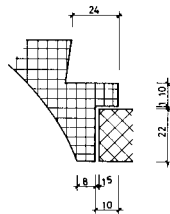
DETAIL ANTRITT
