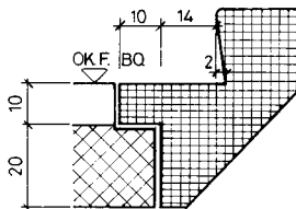
DETAIL ANTRITT
