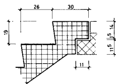
DETAIL AUSTRITT
