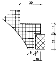
DETAIL ANTRITT
