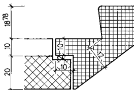
DETAIL ANTRITT
