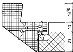
DETAIL ANTRITT
