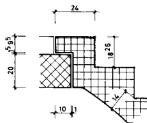
DETAIL AUSTRITT
