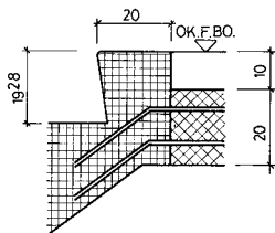
DETAIL AUSTRITT
