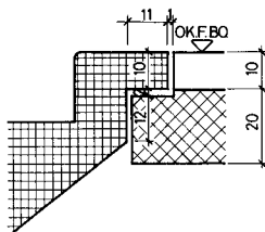
DETAIL AUSTRITT
