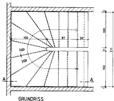
DETAIL ANTRITT
