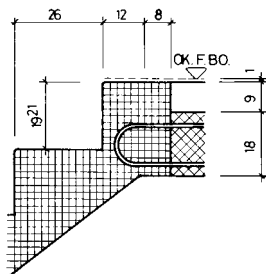
DETAIL AUSTRITT
