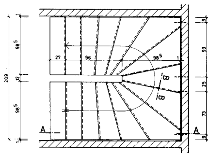
DETAIL ANTRITT
