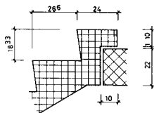
DETAIL AUSTRITT
