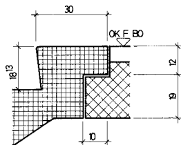
DETAIL AUSTRITT
