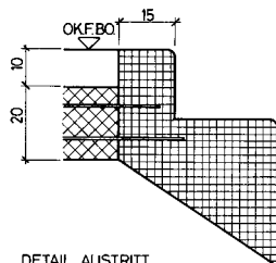
DETAIL AUSTRITT
