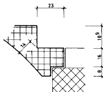
DETAIL ANTRITT
