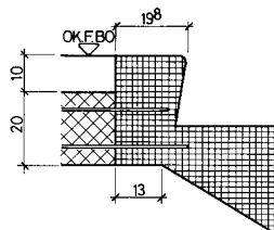
DETAIL AUSTRITT
