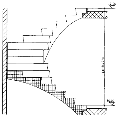
DETAIL AUSTRITT
