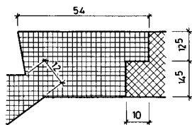
DETAIL AUSTRITT
