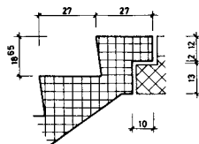
DETAIL AUSTRITT
