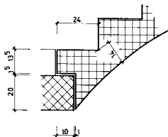
DETAIL ANTRITT
