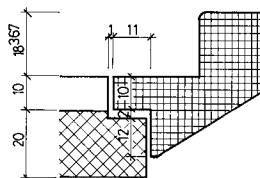
DETAIL ANTRITT
