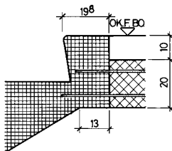
DETAIL AUSTRITT
