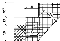
DETAIL ANTRITT
