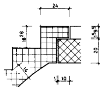
DETAIL AUSTRITT
