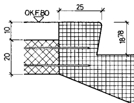
DETAIL AUSTRITT
