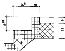
DETAIL AUSTRITT
