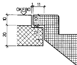
DETAIL AUSTRITT
