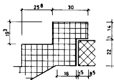
DETAIL AUSTRITT
